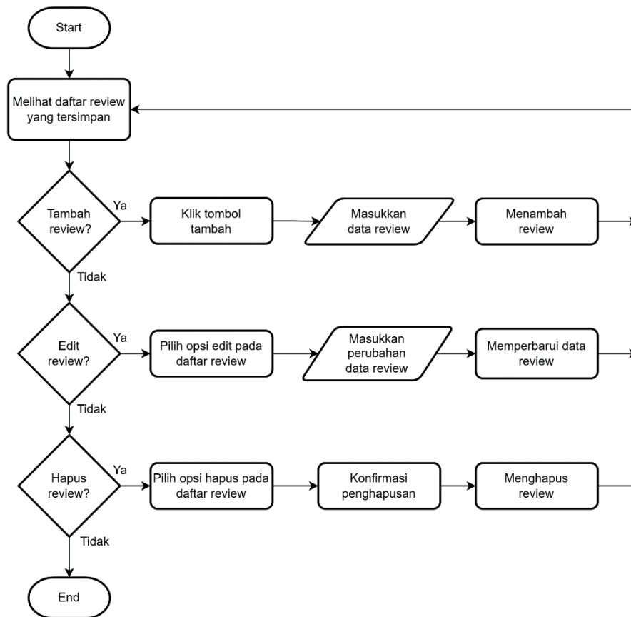
Gambar I - 8. Flowchart Review
