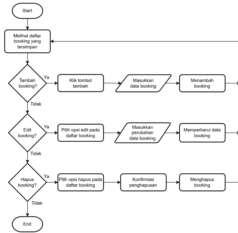
Gambar I - 4. Flowchart Booking
