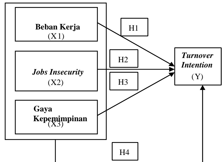
Gambar 1. Model Empiris
