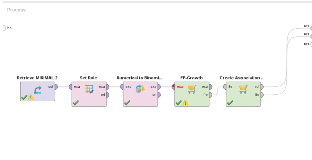
Lampiran 4 Alur Rapid Miner
