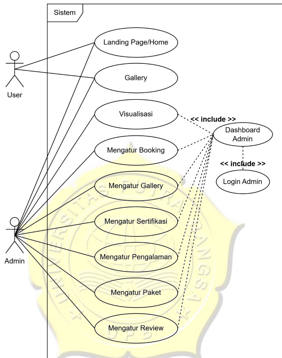
Gambar I - 11. Use Case
