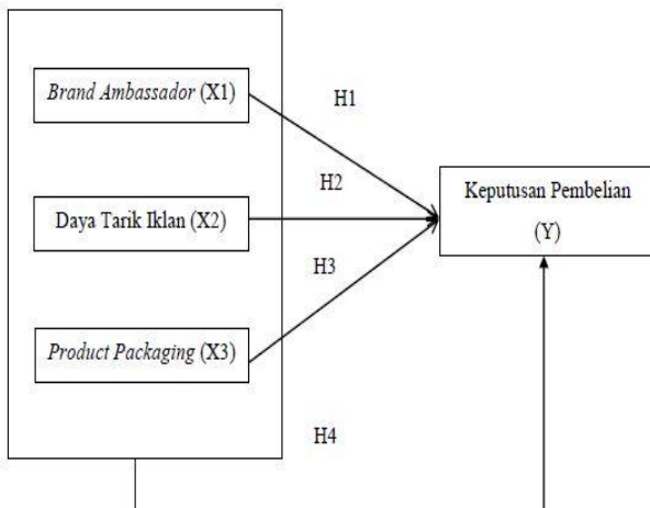
Gambar 3. Model Penelitian
